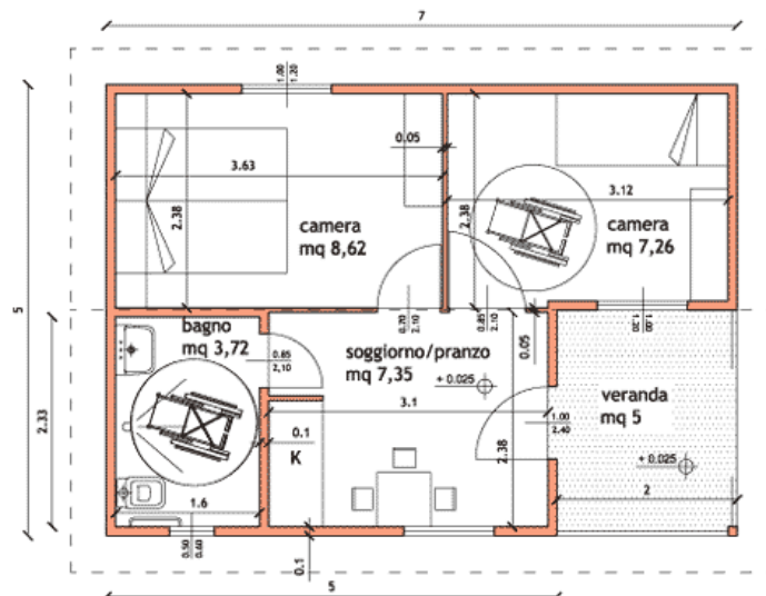
Type BH: 35 m 2 (equipped for the disabled) - 4 beds - living room/kitchenette, 1 room with double bed + room with bunk bed, bathroom and veranda;
