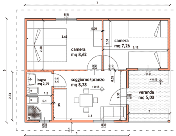
Type B: 35 m 2 - 5 beds - living room/kitchenette, 2 bedrooms (1 room with double bed + 1 room with bunk bed + pullout bed), bathroom and veranda;
